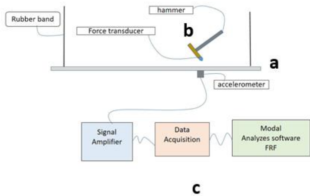
Fig. 1. Experimental modal testing setup for the free-free aluminum beam: (a) overall view of the suspended beam using elastic cords to simulate free-free boundary conditions, (b) location of the calibrated impact hammer and the single axis accelerometer mounted with wax at the reference point, and (c) connection to the amplifier and data acquisition system.
