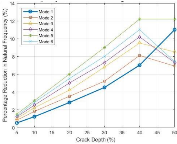
Fig. 2. Percentage reduction in the natural frequencies of the six bending modes in the presence of a transverse crack with various depths (5% to 50%).
