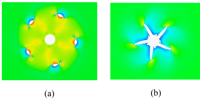
Fig. 2. Comparison of pressure coefficient for a) The optimal toroidal propeller and b) The KP505 propeller
