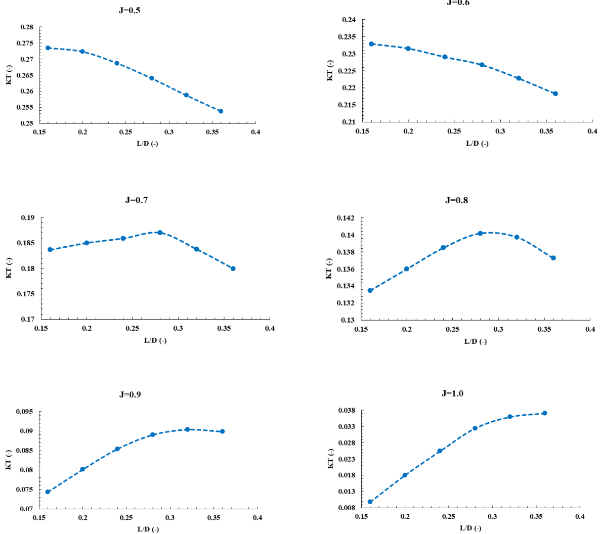
Fig. 10. Changes in thrust coefficient versus spacing ratio for various advance ratios.
