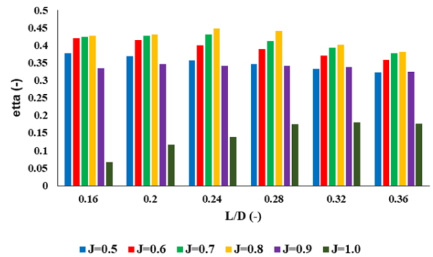
Fig. 1. Propeller efficiency changes versus spacing ratio for various advance ratios.
