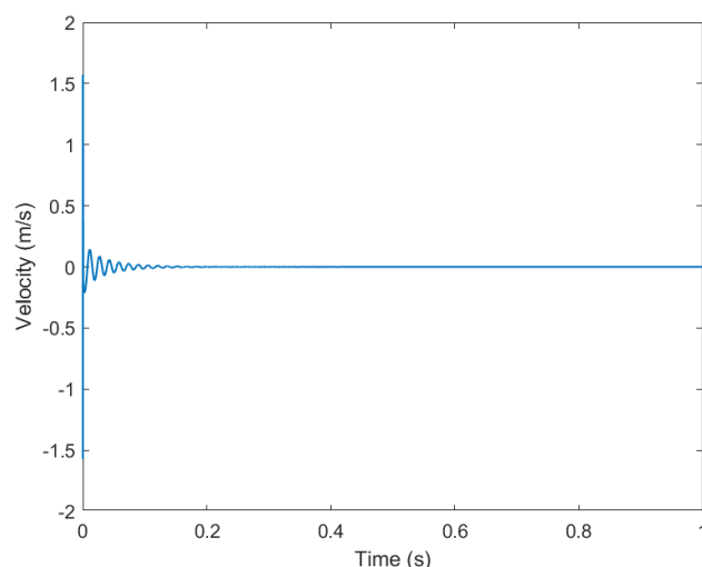
Fig. 3. Linear velocity at the free end of the smart composite beam.
