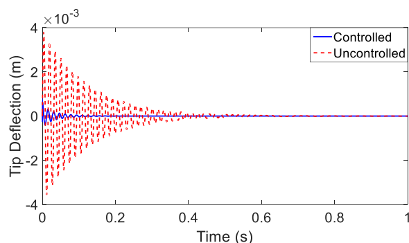
Fig. 2. Dynamic response of the smart composite beam under impulsive loading using fuzzy control.
