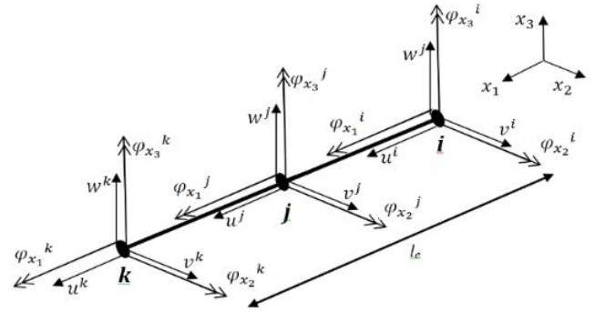
Fig. 1. Three-noded Timoshenko beam element modeling composite box beam with shear and coupling effects..
