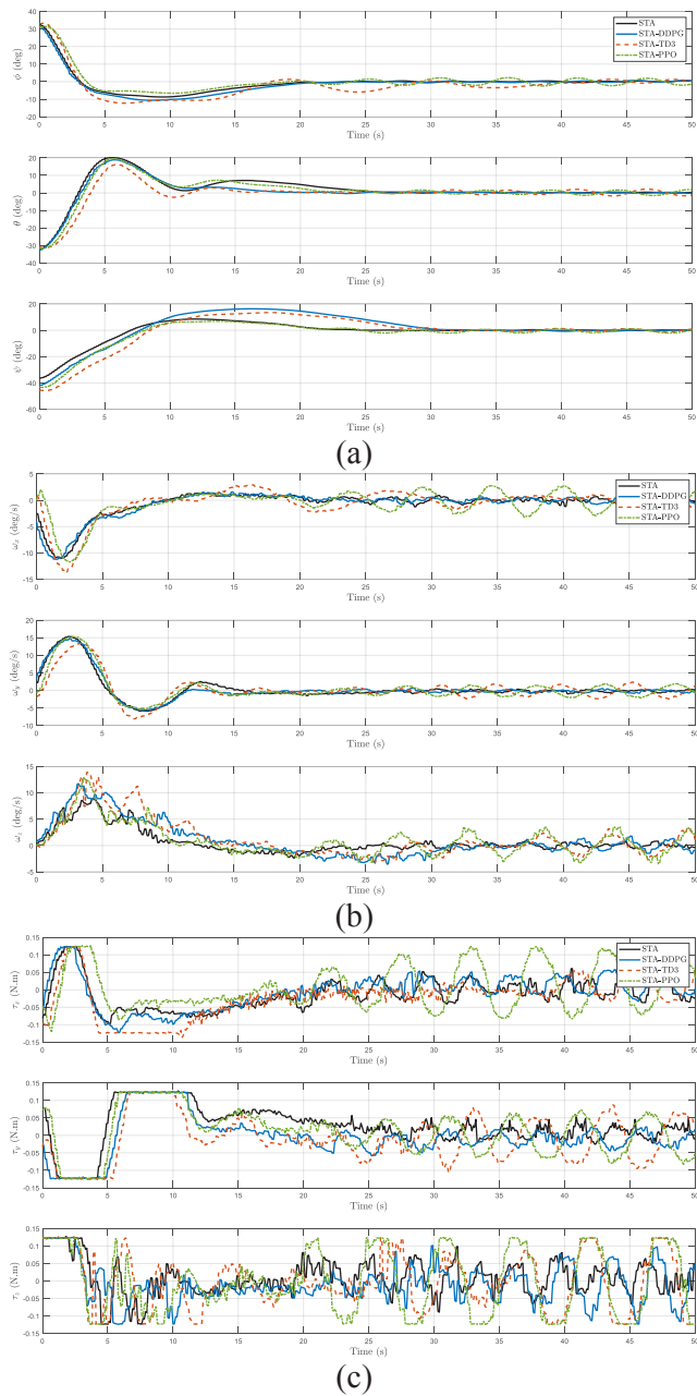
Fig. 2. Experimental implementation results of four control strategies in the presence of inherent test platform disturbances: (a) attitude angles, (b) angular velocities, and (c) control inputs.
