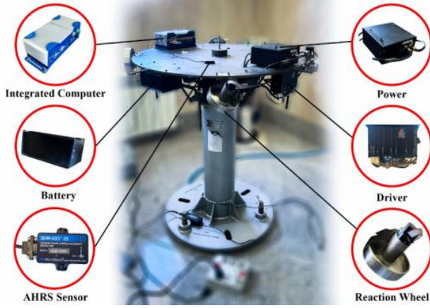
Fig. 1. General structure of the Isfahan University satellite attitude simulator [10].
