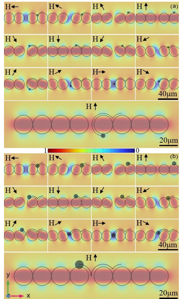
Fig. 2. Simulated trajectories of magnetic microparticles and the corresponding energy distribution on the chip. (a) Non-migrating particle (confined to the original pathway). (b) Migrating particle (crossing the spacing). The arrows indicate the direction of the external magnetic field. The energy values are normalized.
