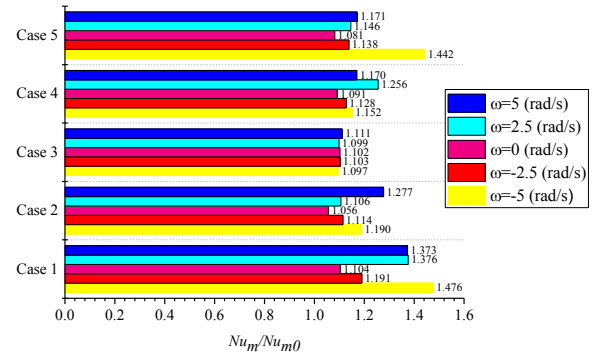
Fig. 2. Ratio of average Nusselt number for various cases for different rotational velocity ( Ra=5 \times 10^5 ).
