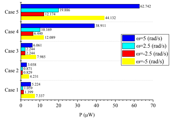
Fig. 3. Power required to rotate the cylinders for various cases for different rotational velocity ( Ra=5 \times 10^5 ).
