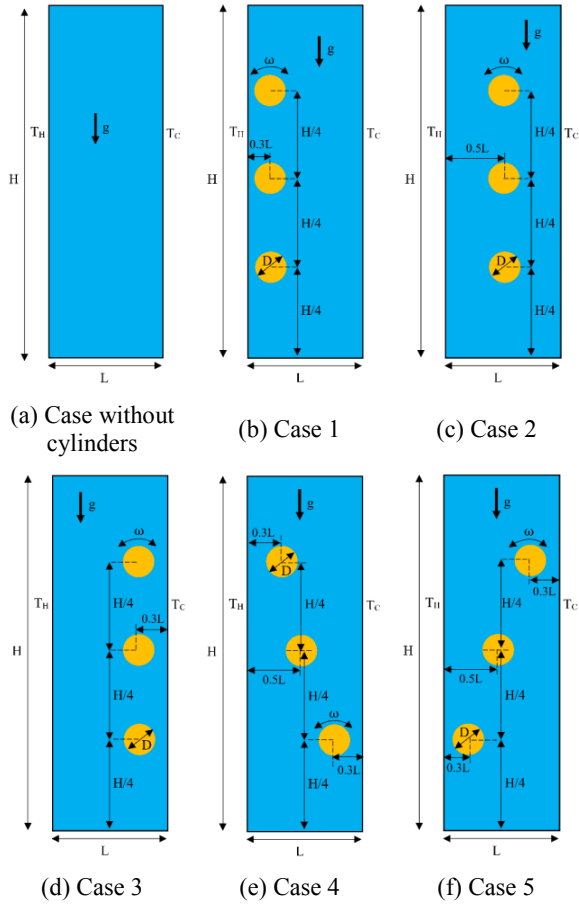
Fig. 1. Schematic representation of the computational geometry.
