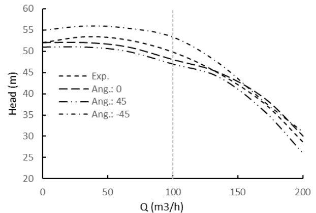
Fig. 1. Comparison of the pump head at three angles ( 0^\circ , 45^\circ , and -45^\circ ) with experimental results.
