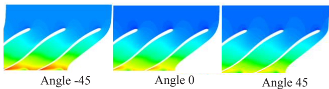
Fig. 2. Static pressure contour in the impeller in three angle positions (0°, 45°, and -45°)
