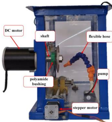
Fig. 1. Main components of the electrochemical grinding apparatus used in the experimental investigation.
