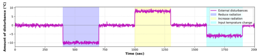
Fig. 6. Amount of disturbance applied to the system.
