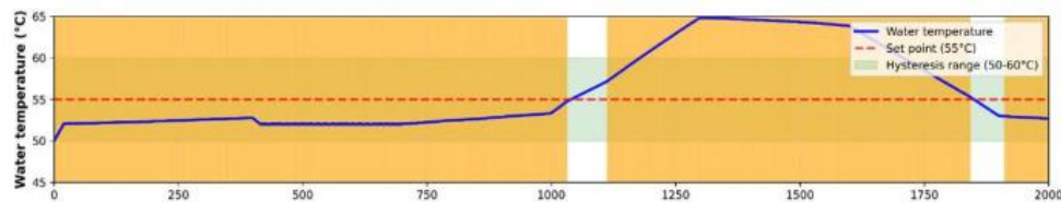
Fig. 3. Graph of changes in water outlet temperature over time.
