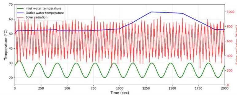
Fig. 8. Changes in inlet and outlet water temperatures and solar radiation versus time.
