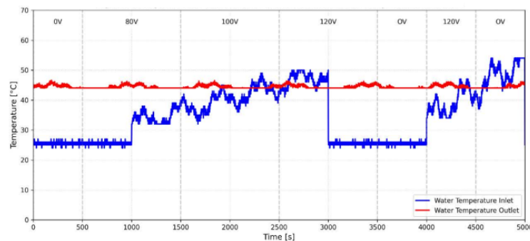
Fig. 7. Testing the controller for changes in inlet and outlet water temperatures.
