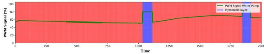
Fig. 4. Temperature changes versus PWM signal.
