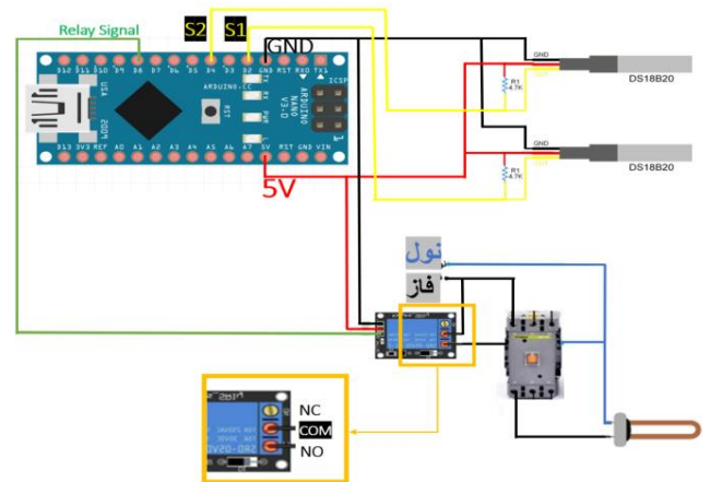
Fig. 2. Schematic of the control circuit designed in Fritzing software.
